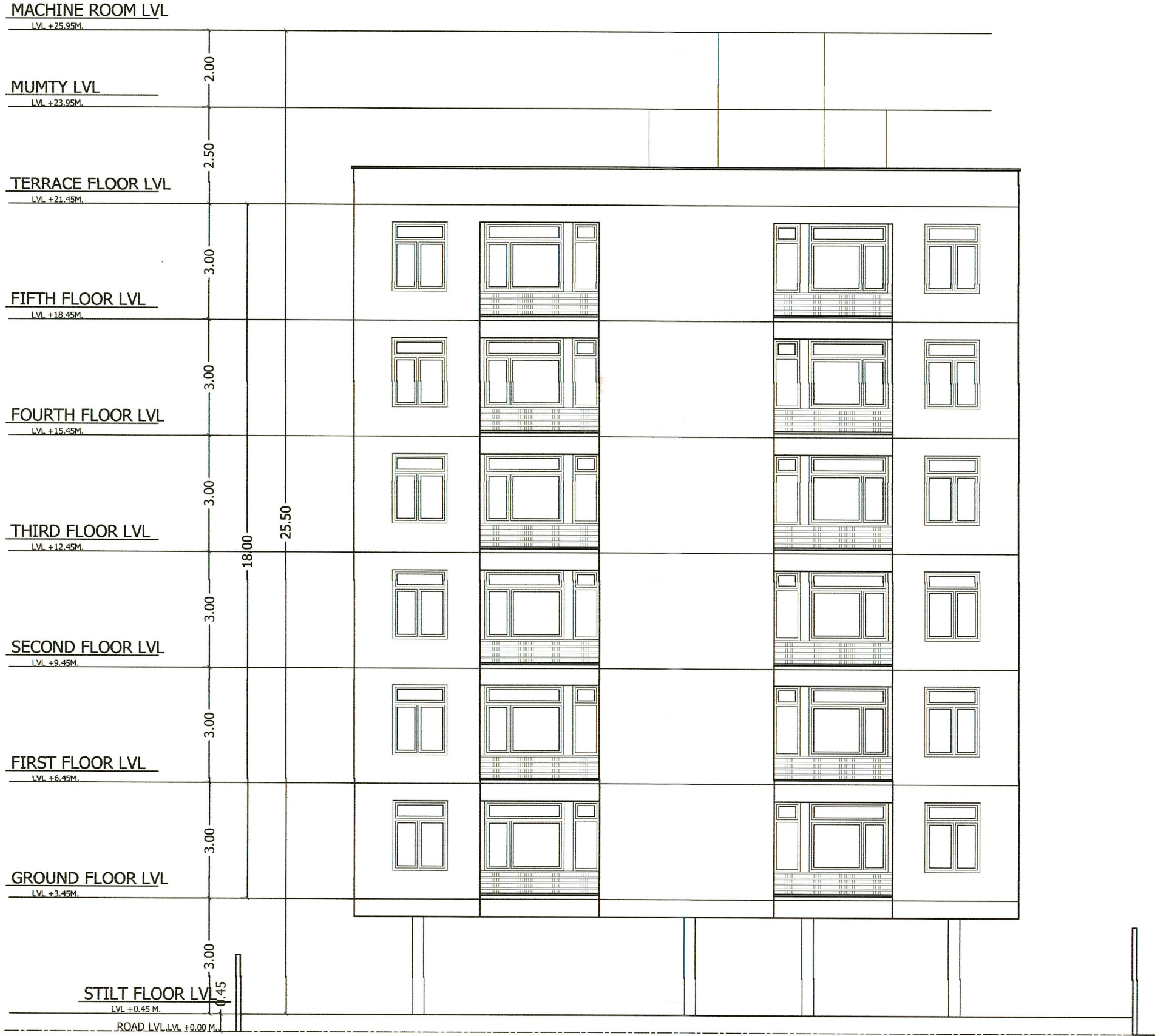
NORTH SIDE ELEVATION
