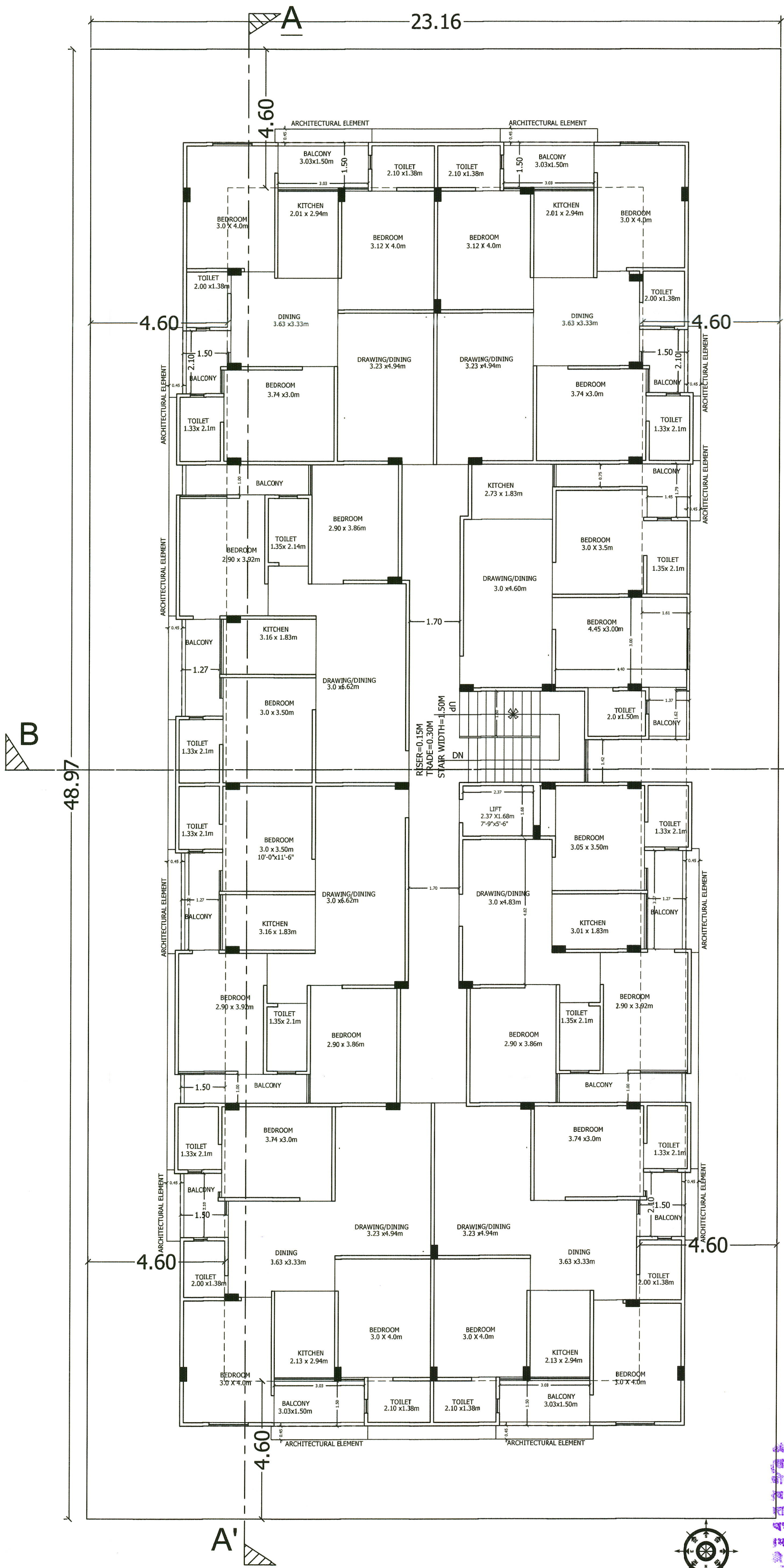
TYPICAL FLOOR PLAN
