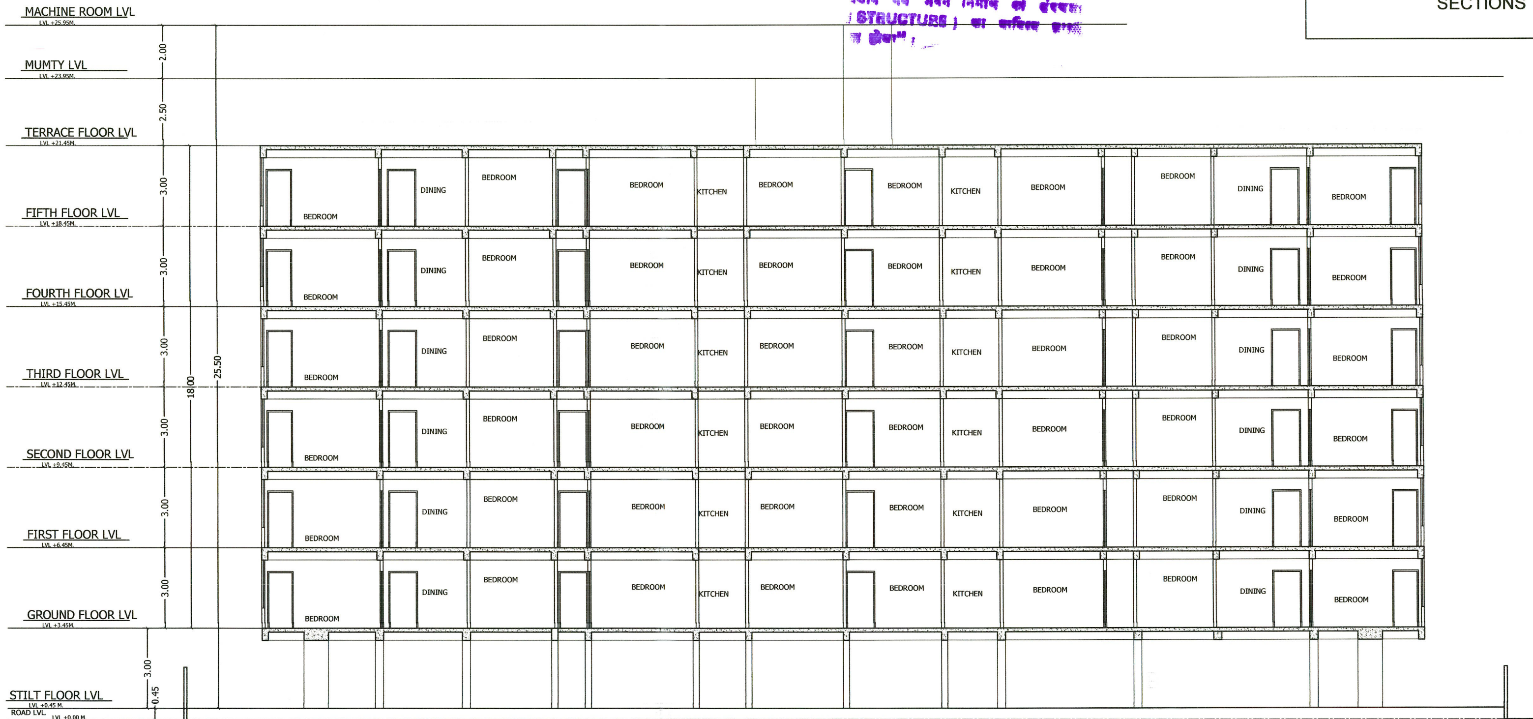
SECTION @ A-A'
