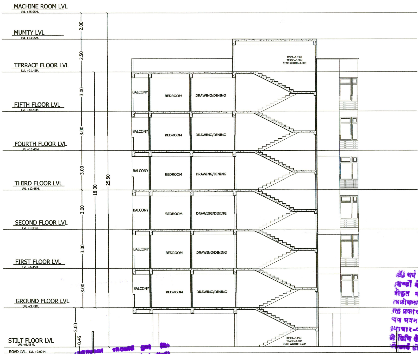
SECTION @ B-B'
