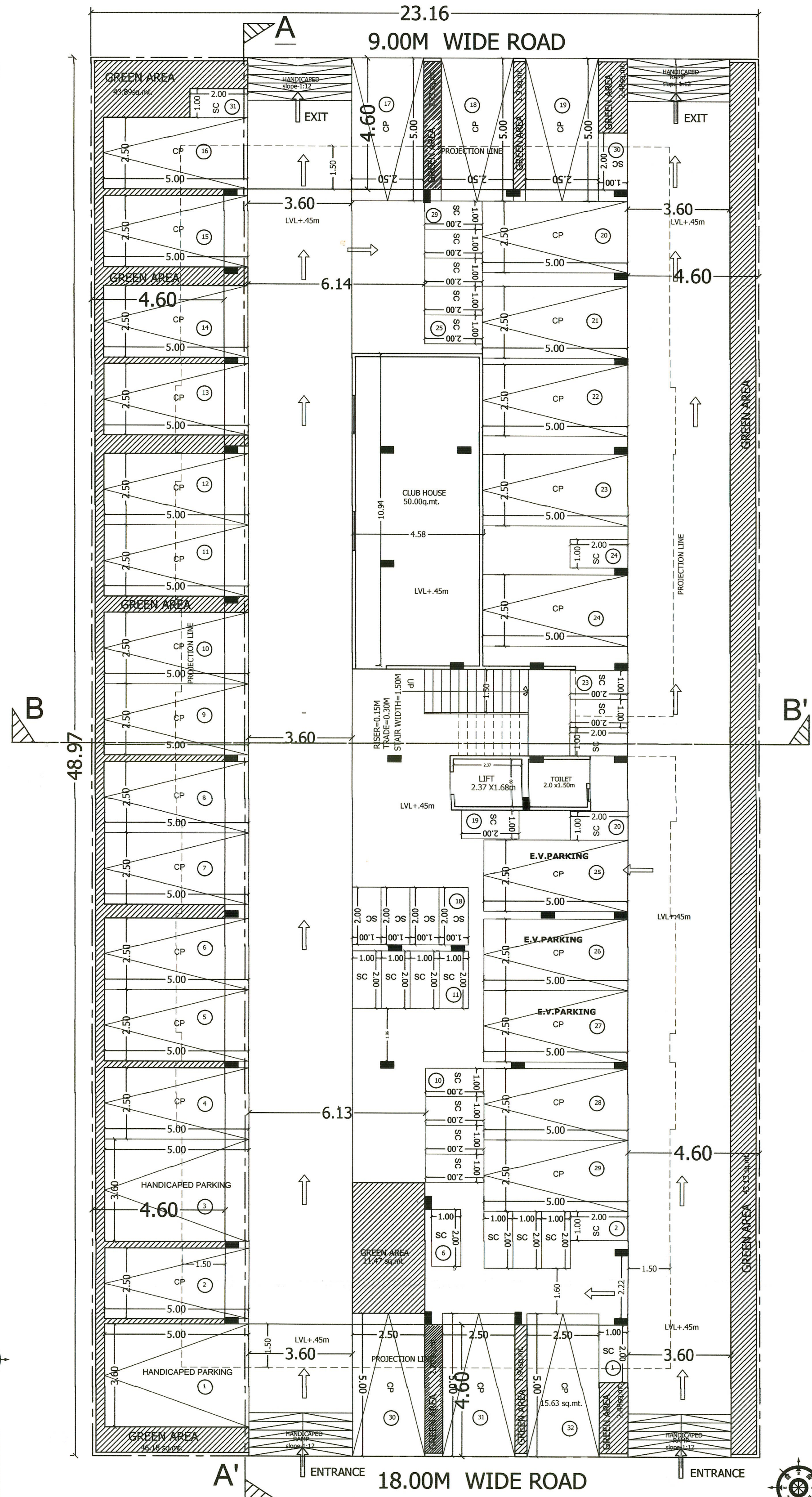
STILT FLOOR PLAN
